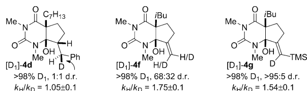
Figure 2. Reductive coupling of barbituric acids 3d , 3f , and 3g using SmI_2/D_2O (only products are shown).
