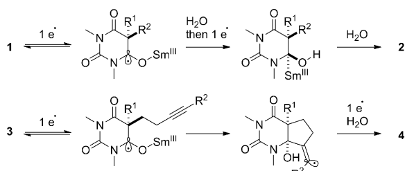
Scheme 1. Mechanism of the reduction and cyclization of barbituric acids using SmI_2/H_2O .
