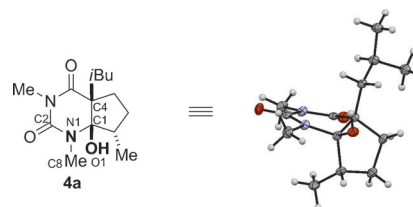
Figure 3. X-ray structure of 4a . Selected bond lengths [ \text{\AA} ] and angles [ ^\circ ]: N1–C1 1.466, C1–O1 1.407, C1–C4 1.552, C1–H1 0.84, N1–C2 1.354, C2–O2 1.218, N2–C2 1.421; C2–N1–C1–O1 155.1, C8–N1–C1–O1 –40.6, N1–C1–O1–H1 –52.1, C4–C1–O1–H1 70.8, C1–N1–C2–N2 –6.9, C2–N2–C3–C4 –14.6, N1–C2–N2–C3 –3.6. [23]
